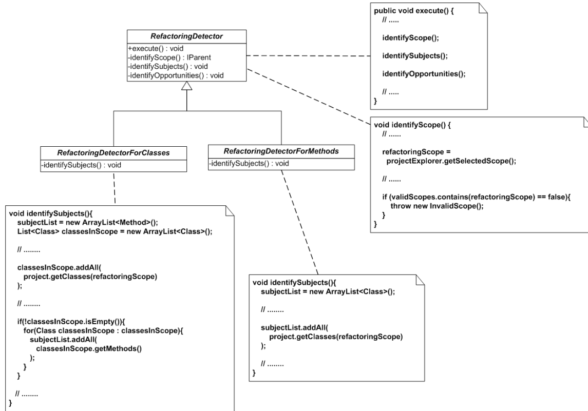
Figure 2: Pattern participants.
