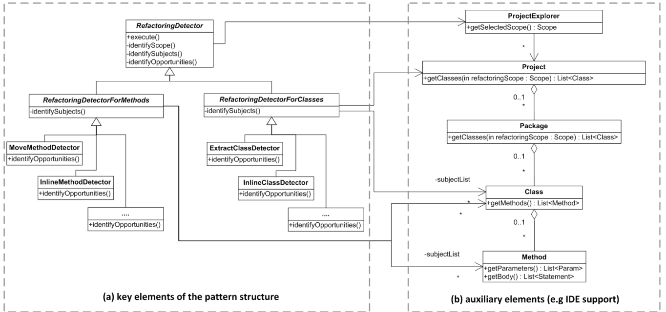
Figure 1: Pattern structure.
