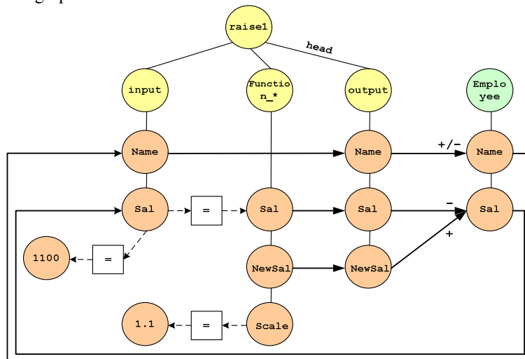
Fig. 2 Side-effects over the LDL++ rule of Fig. 1
