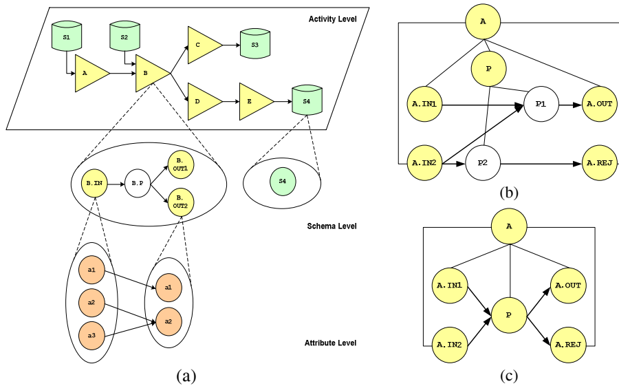
Fig. 4 Zooming in/out. (a) different levels of detail for ETL workflows; (b) an activity with two input schemata populating an output and a rejection schema as follows: a subprogram P1 is assigned the population of the output schema only and a subprogram P2 populates only the rejection schema using only one input schema; and (c) a single node abstracts the internal structure of the activity
