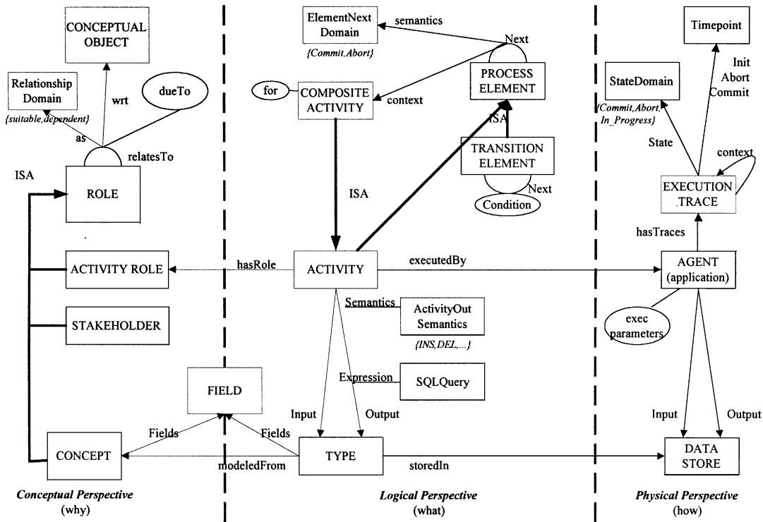
Fig. 6. The metamodel for data warehouse operational processes.
