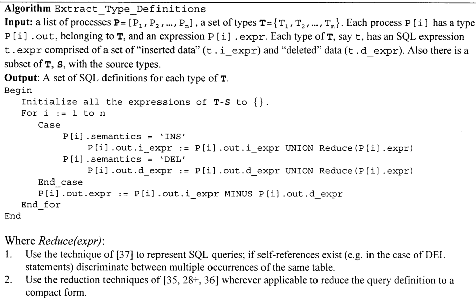
Fig. 18. Algorithm for extracting the definition of a type in the repository.
