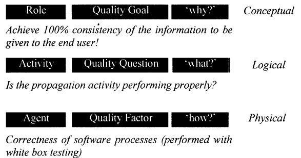
Fig. 16. Perspectives and interrelationships for the process and quality metamodels.
