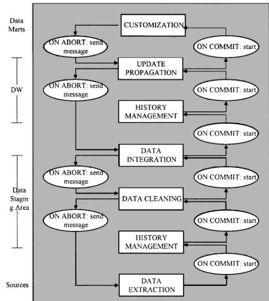
Fig. 4. The Data Warehouse Refreshment process [14].
