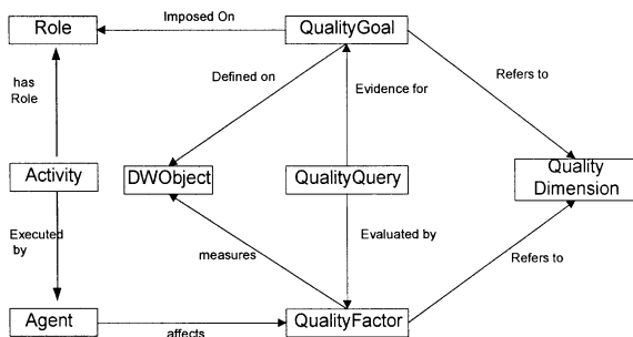
Fig. 15. Relationships between processes and quality.
