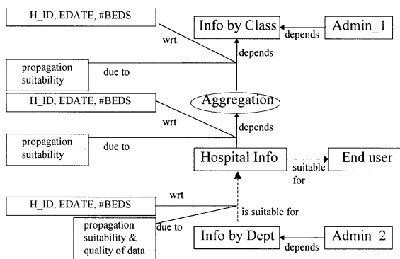
Fig. 11. The conceptual perspective for the example.
