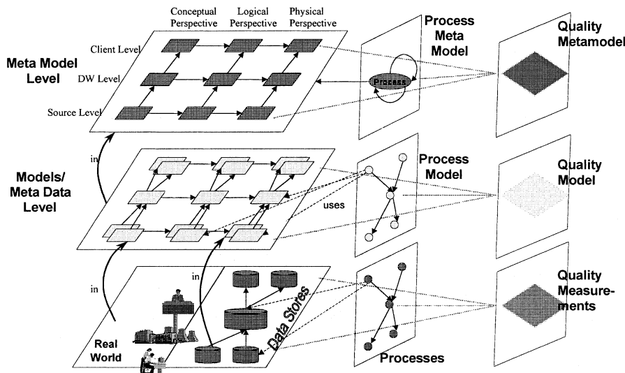
Fig. 2. Framework for Data Warehouse Architecture [1].
