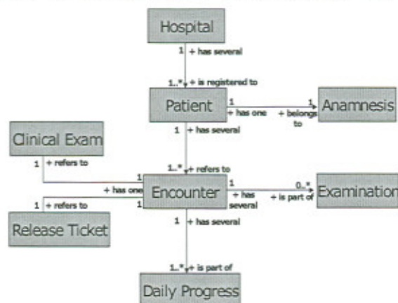
Fig. 2. CPR entities and relations
