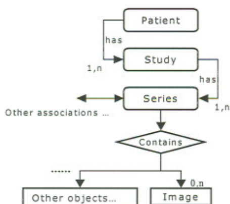
Fig. 1. The core of DICOM Information Model
