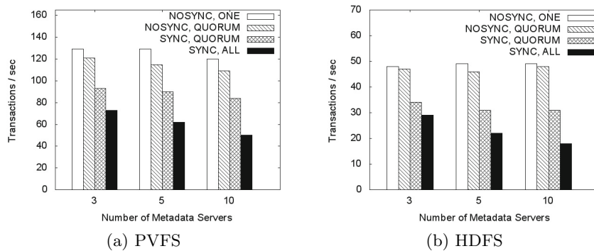
Fig. 6. Postmark throughput for different replication factors
