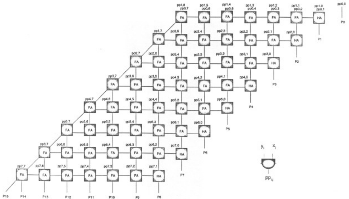
FIGURE 1 An 8-bit carry-propagate array multiplier (CPAM).
