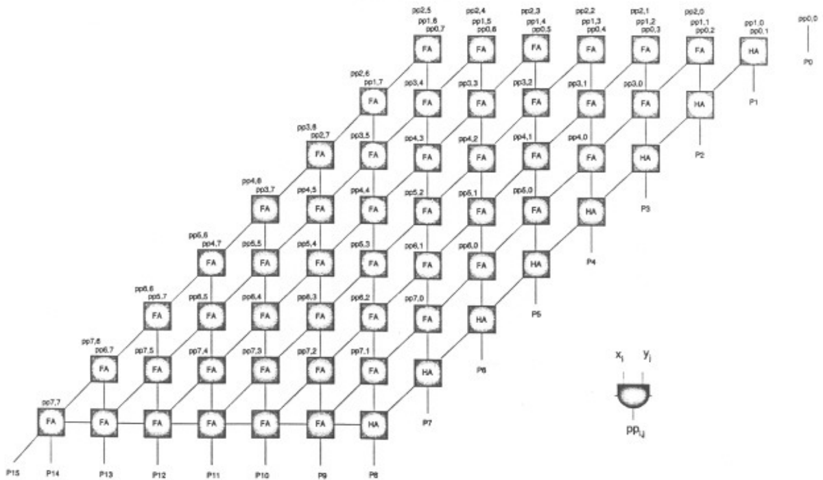
FIGURE 2 An 8-bit carry-save array multiplier (CSAM).
